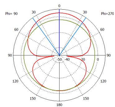
E-plane (Horwin AD 1601)
